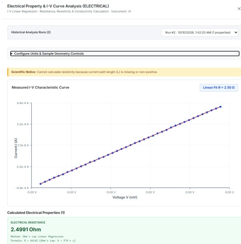
Figure 5.9: Electrical Property and Current-Voltage ( I - V ) Transport Analysis Interface: Experimental I - V characteristic curve exhibiting Ohmic linearity, linear regression slope ( R = 2.50 \Omega ), and automated resistance ( 2.4991 \Omega ) and conductivity calculation.
