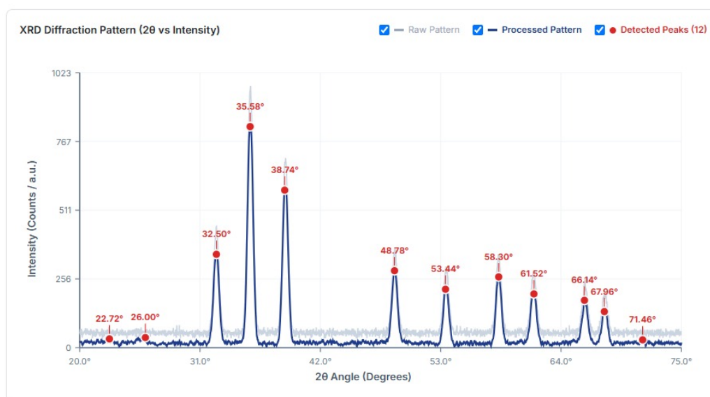
Figure 5.4: X-Ray Diffraction (XRD) Diffractogram Analysis Interface: Interactive 2\theta vs. Intensity pattern visualization showing raw background trace, Savitzky-Golay smoothed curve, and automated detection of 12 Bragg reflection peaks ( 32.50^\circ , 35.58^\circ , 38.74^\circ , 48.78^\circ , 53.44^\circ , 58.30^\circ , 61.52^\circ , 66.14^\circ , 67.96^\circ , 71.46^\circ ).
